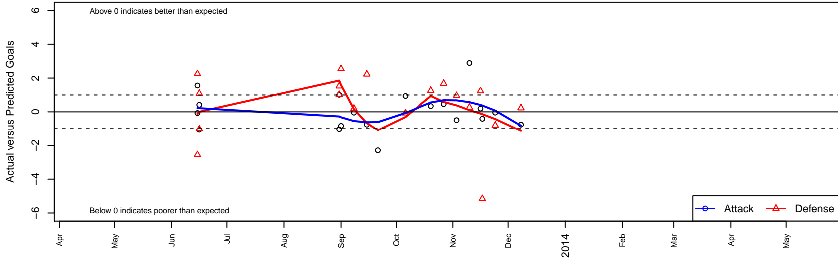
NW United Savoy B96 Dots are actual minus expected GF (blue circles) and GA (red triangles). Blue line is smoothed change in attack strength. Red is smoothed change in defense strength.
